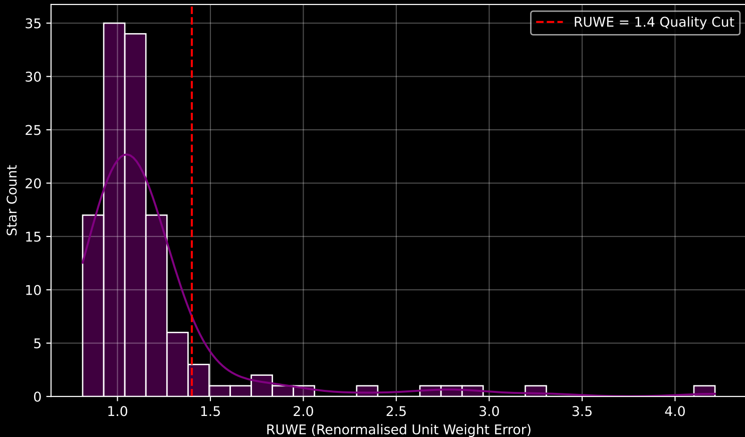
GALAH DR4 Field [6790] RUWE Distribution (n= 124)
