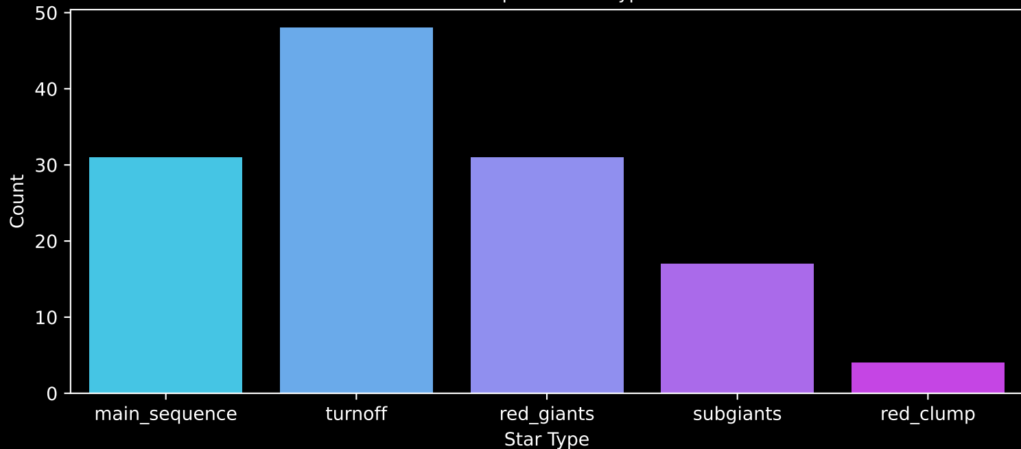
GALAH DR4 Field: [6790] Count plot of Star Type
