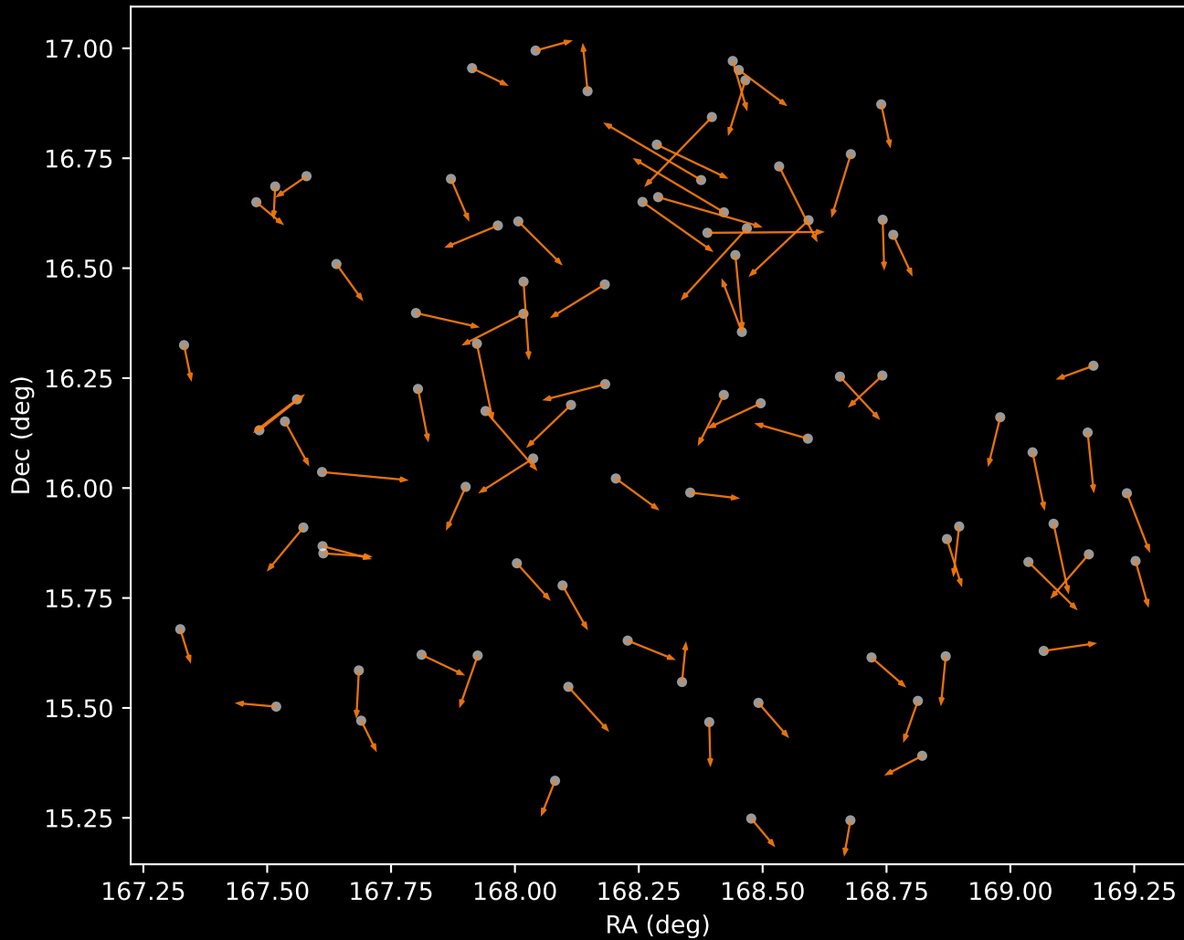
GALAH DR4 Cluster 2 Proper Motion Vectors (n=87)
