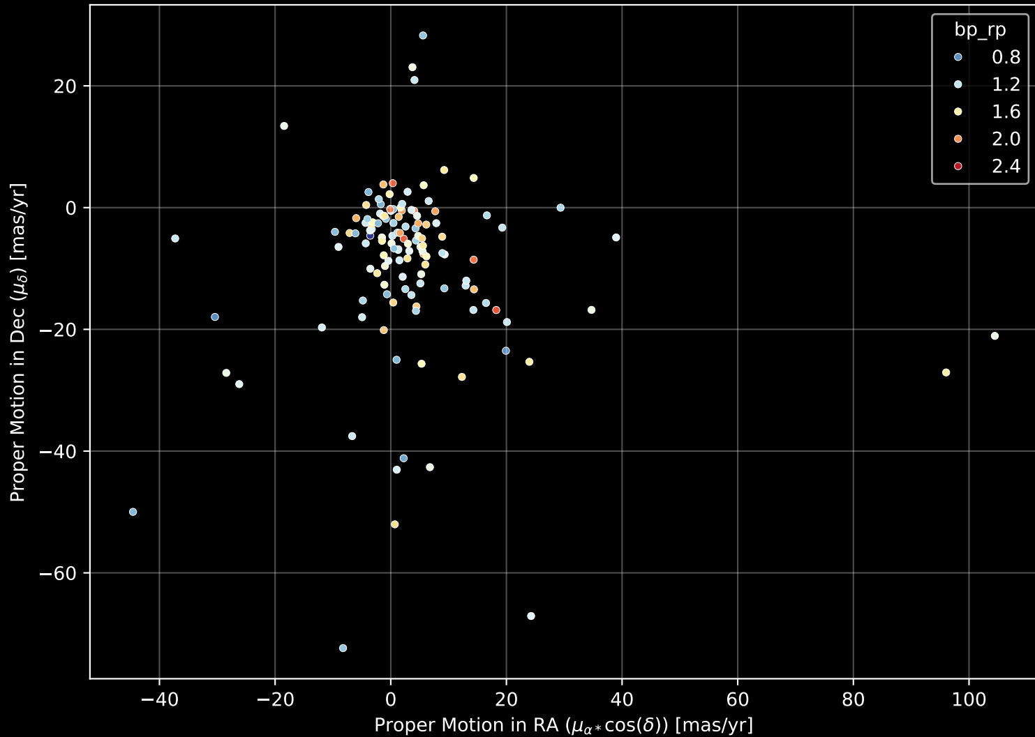
GALAH DR4 Field: [6790] Proper Motion Diagram (n= 131)
